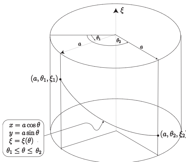
Figure 7.20: A curve that lies entirely on a circular cylinder of radius a , beginning (in circular cylindrical coordinates) at (a, \theta_1, \xi_1) and ending at (a, \theta_2, \xi_2) .
