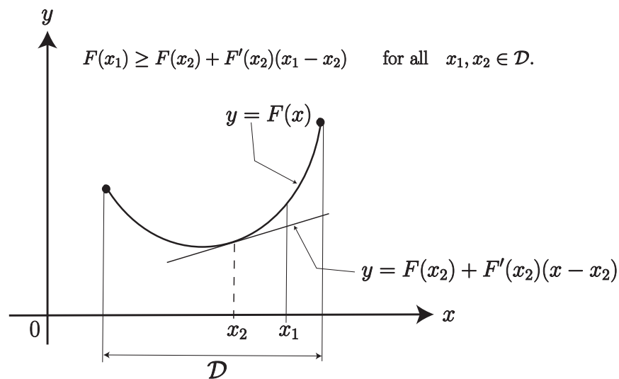
Figure 7.19: A convex curve y = F(x) lies above the tangent line through any point of the curve.
