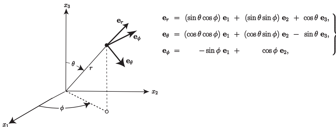
Figure 6.4: Spherical coordinates (r, \theta, \phi) and the associated local curvilinear orthonormal basis \{\mathbf{e}_r, \mathbf{e}_\theta, \mathbf{e}_\phi\} .
