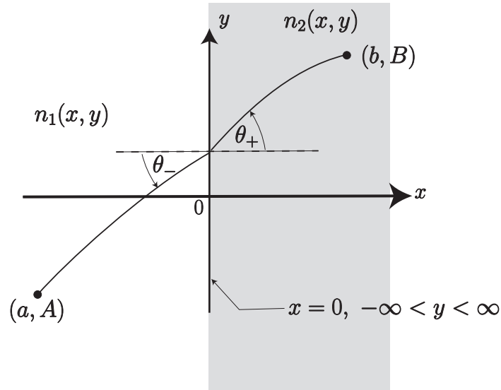
Figure 7.12: Ray of light in a two-phase material.
