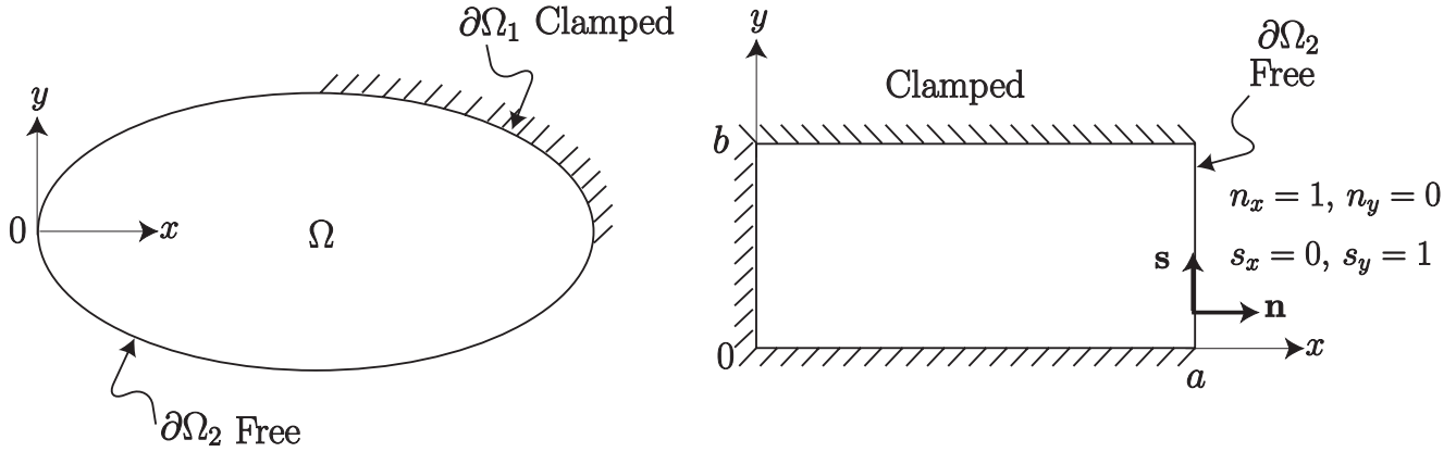
Figure 7.17: Left: A thin elastic plate whose mid-plane occupies a region \Omega of the x, y -plane. The segment \partial\Omega_1 of the boundary is clamped while the remainder \partial\Omega_2 is free of loading. Right: A rectangular a \times b plate with a load free edge at its right hand side x = a, 0 \leq y \leq b .
