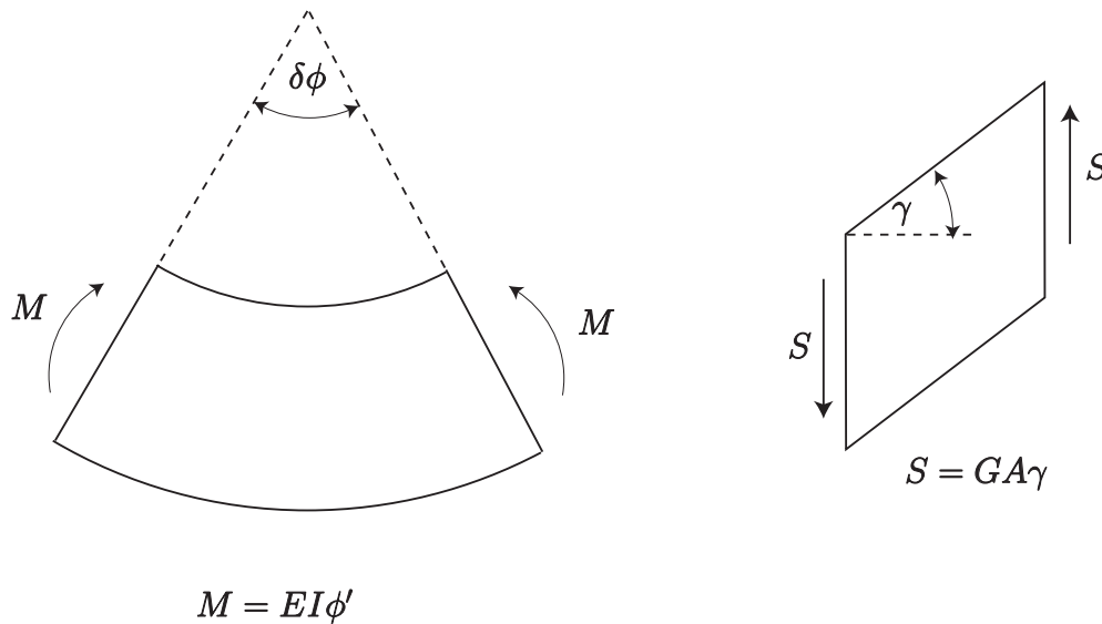
Figure 7.8: Basic constitutive relationships for a beam.
