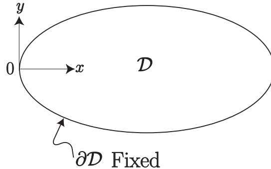
Figure 7.15: A stretched elastic membrane whose mid-plane occupies a region \mathcal{D} of the x, y -plane and whose boundary \partial\mathcal{D} is fixed. The membrane surface is subjected to a pressure loading p(x, y) that acts in the negative z -direction.
