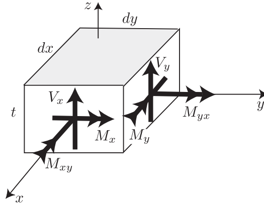
Figure 7.16: A differential element dx \times dy \times t of a thin plate. A bold arrow represents a force and thus V_x and V_y are (shear) forces. A bold arrow with two arrow heads represents a moment whose sense is given by the right hand rule. Thus M_{xy} and M_{yx} are (twisting) moments while M_x and M_y are (bending) moments.
