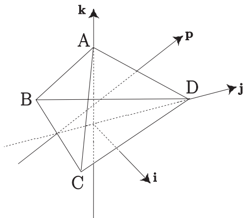
Figure 4.5: A regular tetrahedron ABCD , three orthonormal vectors \{\mathbf{i}, \mathbf{j}, \mathbf{k}\} and a unit vector \mathbf{p} . The axis \mathbf{k} passes through the vertex A and the centroid of the opposite face BCD , while the unit vector \mathbf{p} passes through the center of the edge AD and the center of the opposite edge BC .
