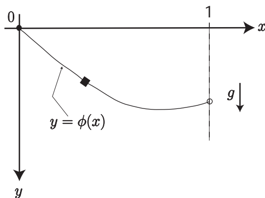
Figure 7.5: Curve joining (0, 0) to an arbitrary point on the vertical line through x = 1 .
