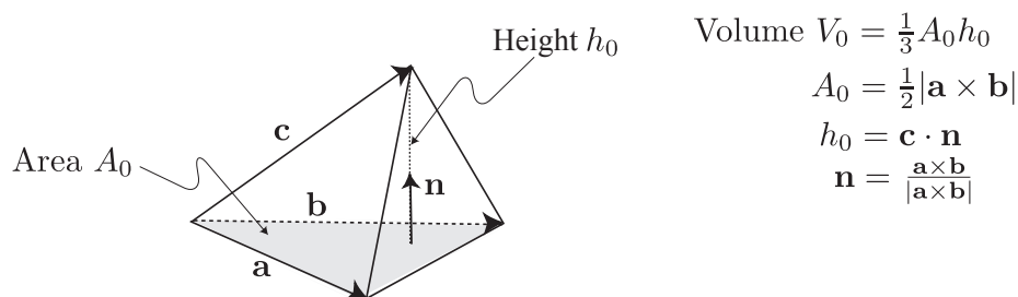
Figure 2.2: Volume of the tetrahedron defined by vectors \mathbf{a}, \mathbf{b}, \mathbf{c} .
