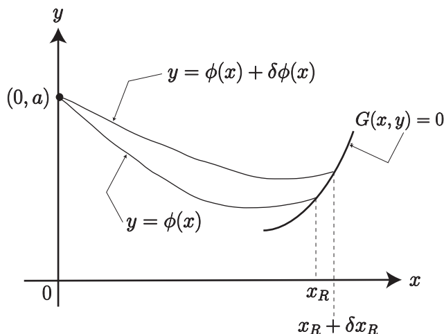
Figure 7.9: Curve joining (0, a) to an arbitrary point on the given curve G(x, y) = 0 .
