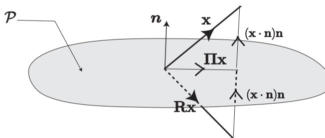
Figure 2.3: The projection \mathbf{\Pi x} and reflection \mathbf{R x} of a vector \mathbf{x} on the plane \mathcal{P} .
