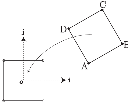
Figure 4.1: Mapping a square into itself.
