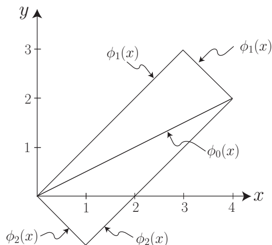
Figure 7.14: Smooth extremal \phi_0(x) and piecewise smooth extremals \phi_1(x) and \phi_2(x) .
