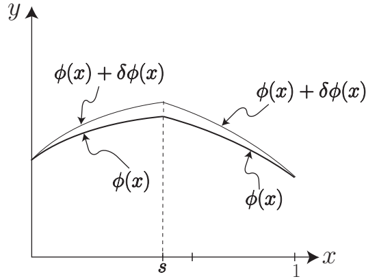
Figure 7.11: Extremal \phi(x) and a neighboring test function \phi(x) + \delta\phi(x) both with kinks at x = s .
