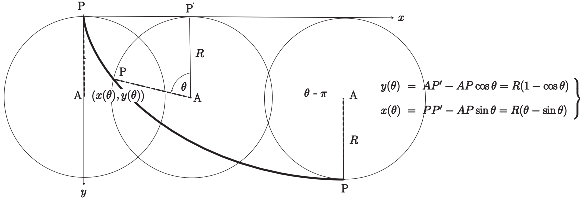
Figure 7.4: A cycloid x = x(\theta), y = y(\theta) is generated by rolling a circle along the x -axis as shown, the parameter \theta having the significance of being the angle of rolling.
