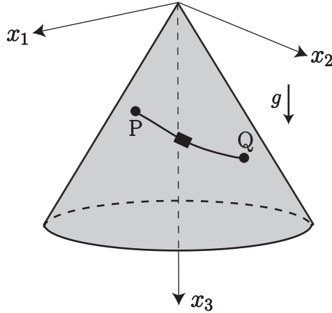
Figure 7.10: A curve that joins the points (p_1, p_2, p_3) to (q_2, q_2, q_3) and lies on the conical surface x_1^2 + x_2^2 - x_3^2 \tan^2 \alpha = 0 .
