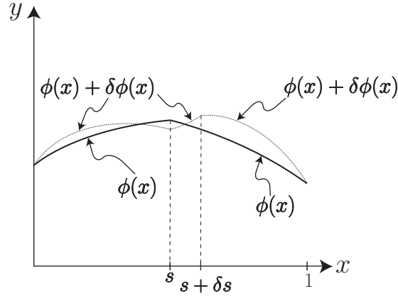
Figure 7.13: Extremal \phi(x) with a kink at x = s and a neighboring test function \phi(x) + \delta\phi(x) with kinks at x = s and s + \delta s .
