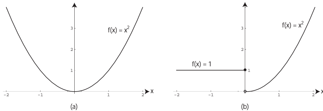
Figure 7.21: (a) The function f(x) = x^2 for -\infty < x < \infty and (b) the function f(x) = 1 for x \leq 0 , f(x) = x^2 for x > 0 .
