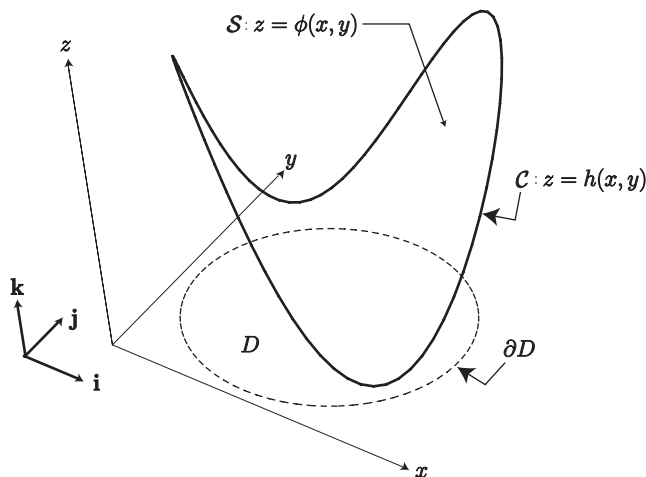
Figure 7.18: The closed curve C in \mathbb{R}^3 is given. From among all surfaces \mathcal{S} in \mathbb{R}^3 that have C as its boundary, the surface with minimal area is to be sought. The curve \partial D is the projection of C onto the x, y -plane.
