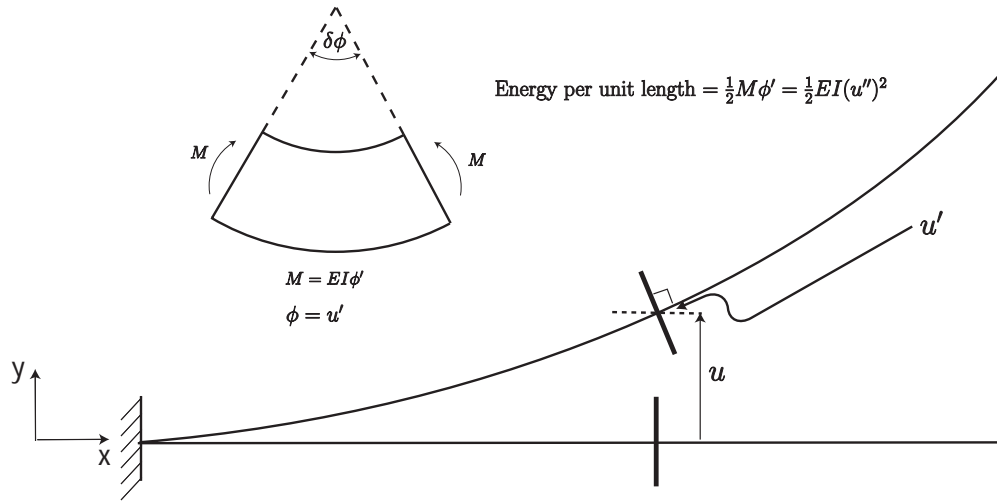
Figure 7.6: The neutral axis of a beam in reference (straight) and deformed (curved) states. The bold lines represent a cross-section of the beam in the reference and deformed states. In the classical Bernoulli-Euler theory of beams, cross-sections remain perpendicular to the neutral axis.
